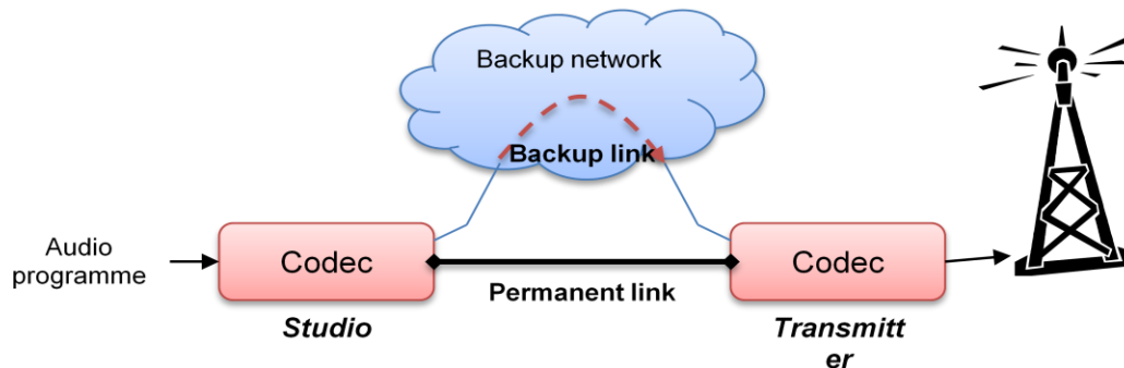
Figure 6 – Backup link
