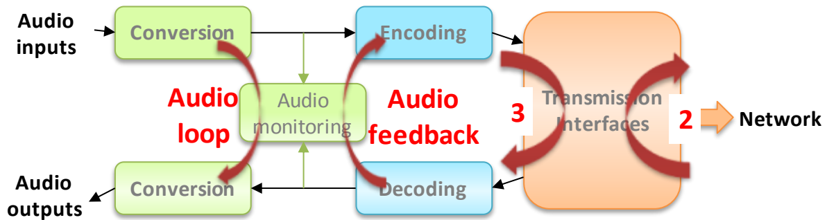
Figure 2 – Test loops
