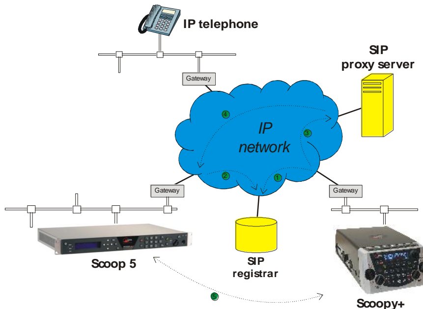
Figure 7 – Setting up an SIP session with server(s)
