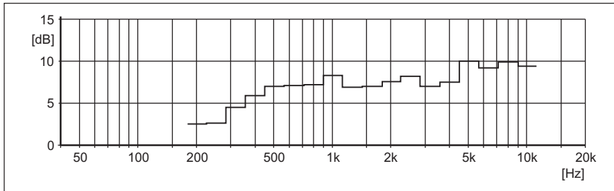
Directivity index
