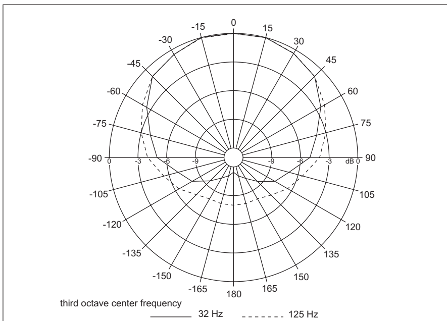
Directional characteristic
