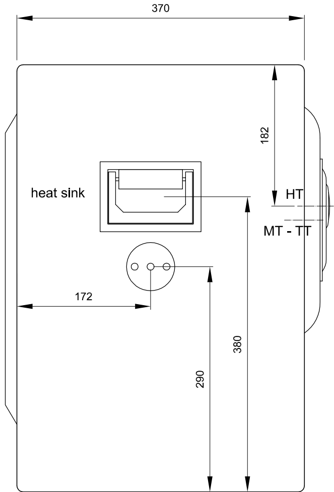
Side view
