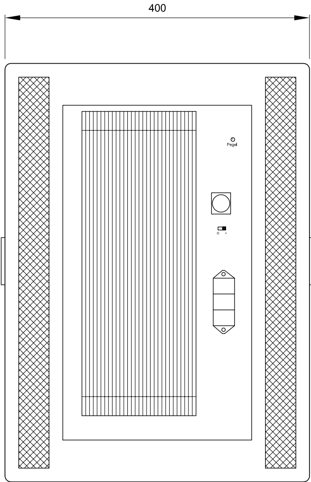
Rear view
