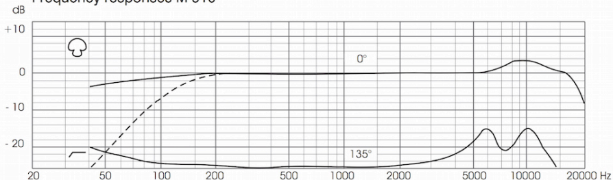
Frequency responses M 910
