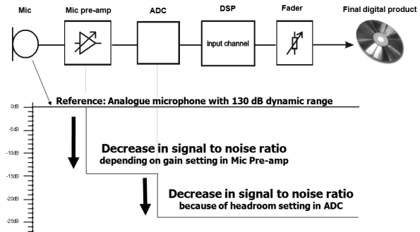
Figure 2 - Decrease in s/n ratio
