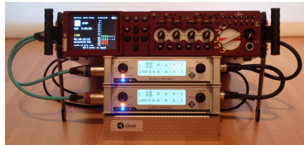
Figure 11 - Current rig: Nagra VI with a pair of Neumann DMI-2Portable for four AES42 microphones powered and clocked from the recorder
