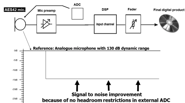
Figure 3 - ADC in the microphone
